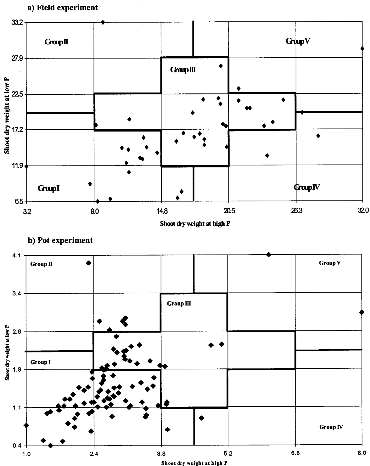
Figure 1. Shoot dry weight variability of cowpea lines to low (no P applied) and high P (60 kg P/ha) application.
