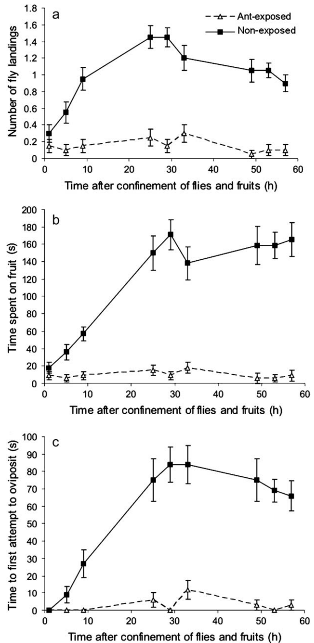
Fig. 1. Effects of cues of Oecophylla longinoda on fruit fly oviposition behaviour. Interactions between treatment and fruit fly species Ceratitidis cosyra and Bactrocera invadens were not significant ( P = 0.05 ), hence data were pooled. (a) Number of fruit fly landings on exposed and unexposed mangoes; (b) time spent per fruit fly walking on exposed and unexposed mangoes; (c) time to first attempt to oviposit by fruit flies on exposed and unexposed mangoes. Oviposition behaviour was significantly lower on mangoes on which predatory ants had patrolled (Student–Newman–Keuls test, n = 20 , P < 0.05 ). Data are the mean \pm SE.
