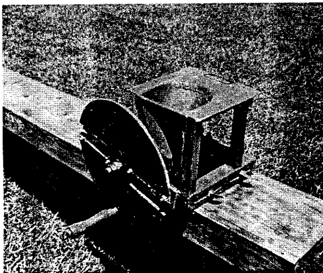
Plate 6. Sweet cassava is chipped using a manual or power chipper.
