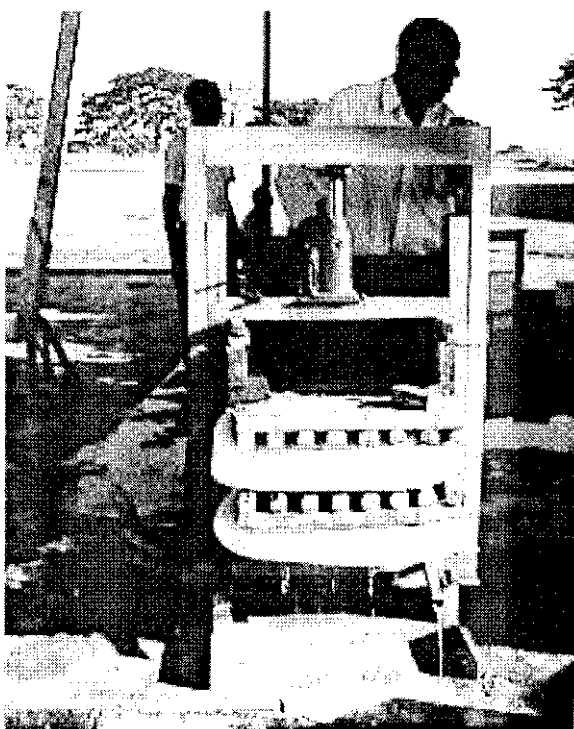
Plate 4. Grated mash is dewatered using a press.
