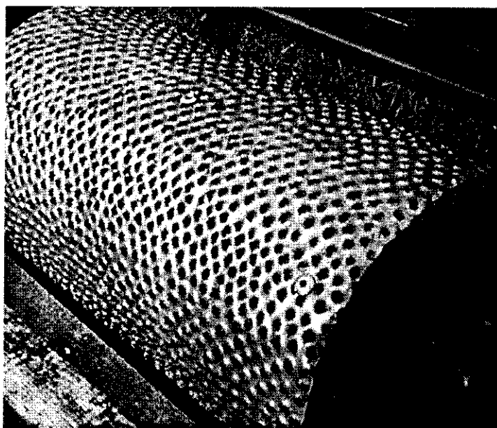
Plate 8. Gari coarse granule rasping head.
