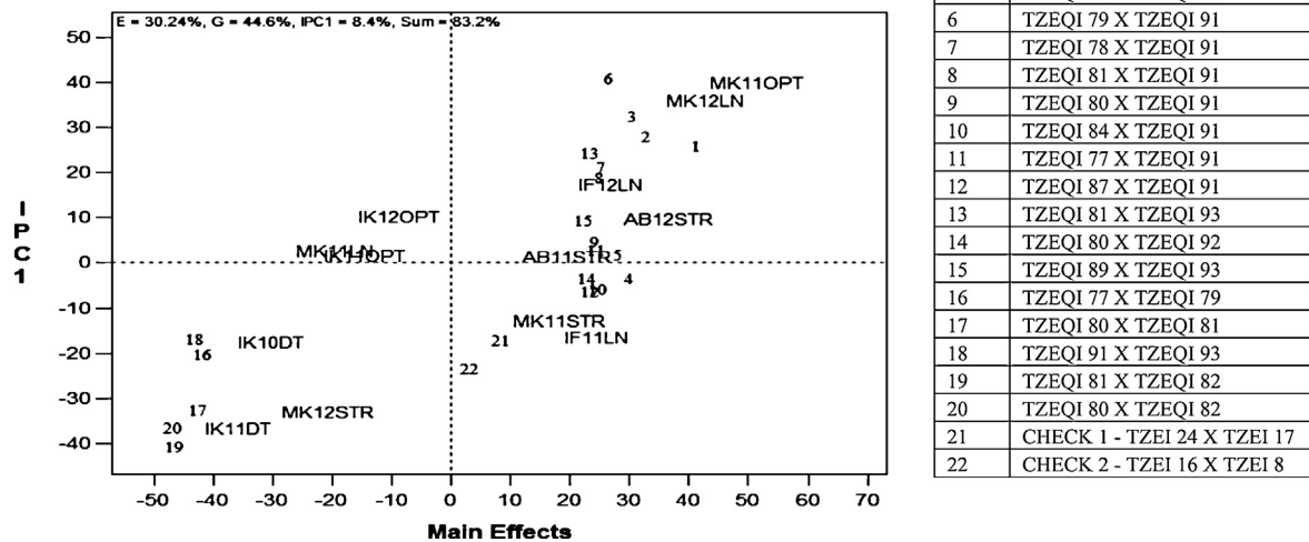
Fig. 2. AMMI biplot of grain yield and the first interaction principal component axis (IPCA 1) of best 15 and worst 5 (based on mean grain yield across environments) early maturing yellow QPM hybrids plus two checks evaluated across 13 environments between 2011 and 2012 in Nigeria. IK11OPT and IK12OPT = Ikenne under optimal growing conditions, 2011 and 2012; IK11DT and IK12DT = Ikenne under drought stress, 2011 and 2012; MK11LN and MK12LN = Mokwa under low N, 2011 and 2012; IF11LN and IF12LN = Ile-Ife under low-N, 2011 and 2012; MK11HN and MK12HN = Mokwa under high-N, 2011 and 2012; IF11HN and IF12HN = Ile-Ife under high-N, 2011 and 2012; MK11STR and MK12STR = Mokwa under Striga infestation, 2011 and 2012; AB11STR and AB12STR = Abuja under Striga infestation, 2011 and 2012.
